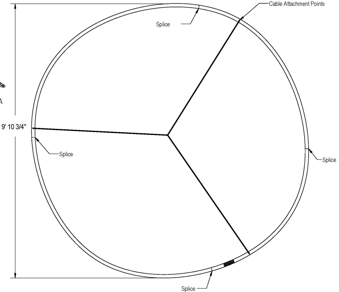
Top View Scale 1 : 16
